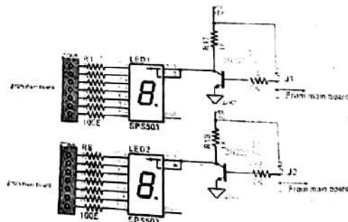
Figure 11.1 Seven Segment LED display connections with controller
