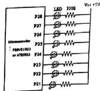
Figure 6.1 LED connections at port 2
